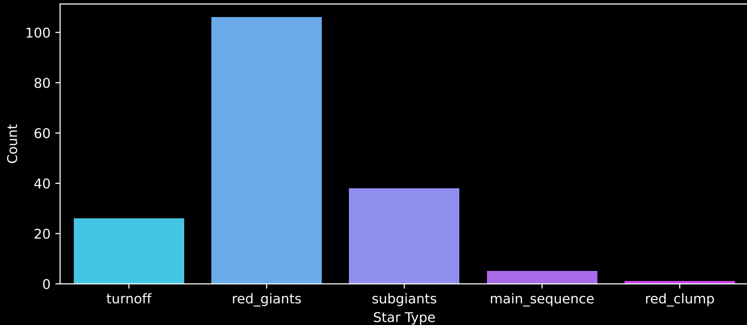
APOGEE DR17 Field: [359+04-O] Count plot of Star Type
