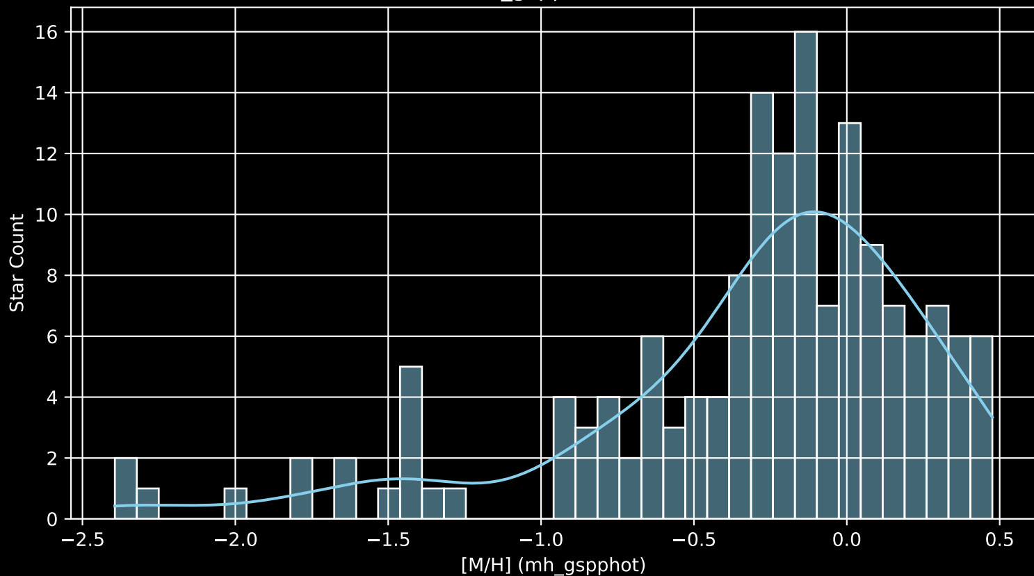
APOGEE DR17 Field: [359+04-O [M/H] (mh_gspphot) (n= 157)
