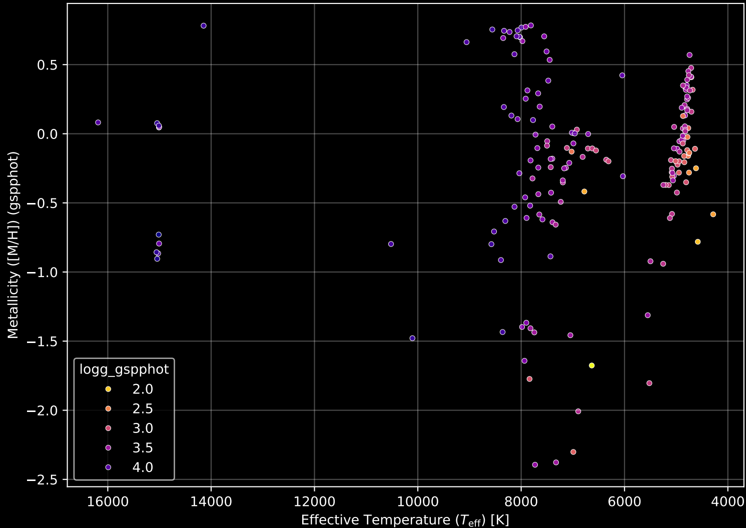
APOGEE DR17 Field: [359+04-O] Stellar Population Parameters (n= 176)
