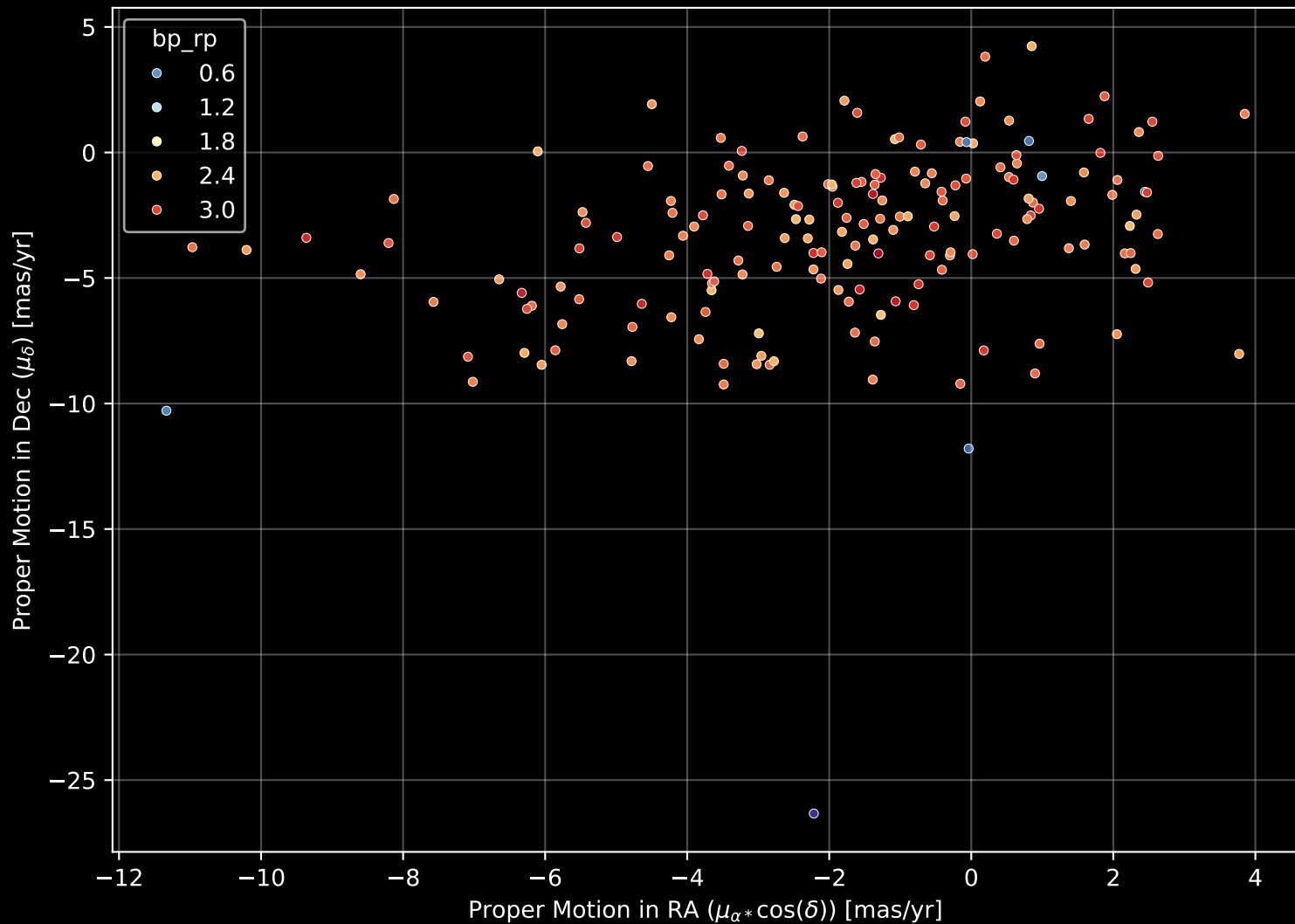
APOGEE DR17 Field: [359+04-O] Proper Motion Diagram (n= 176)
