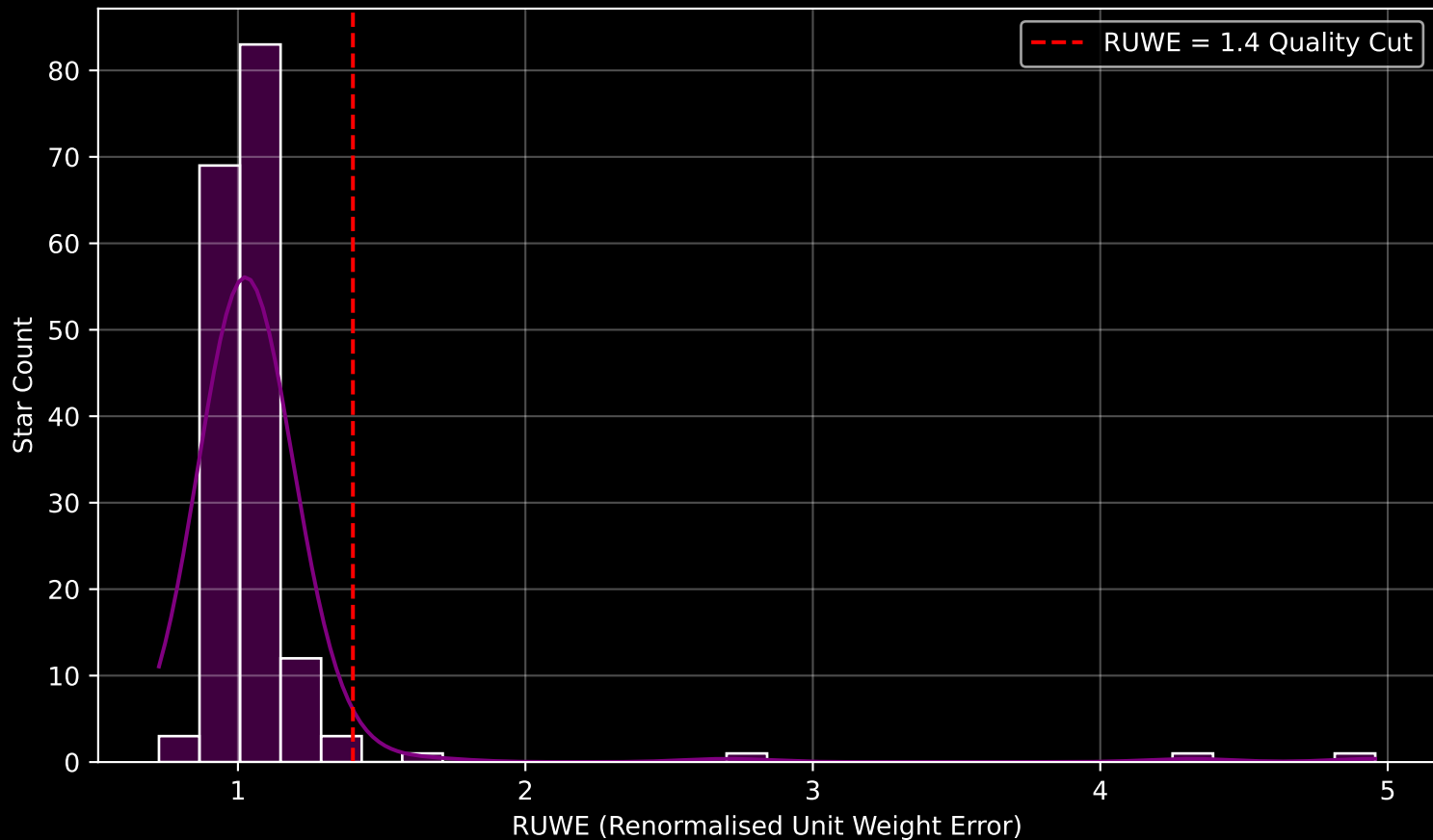
GAPOGEE DR17 Field [359+04-O] RUWE Distribution (n= 174)
