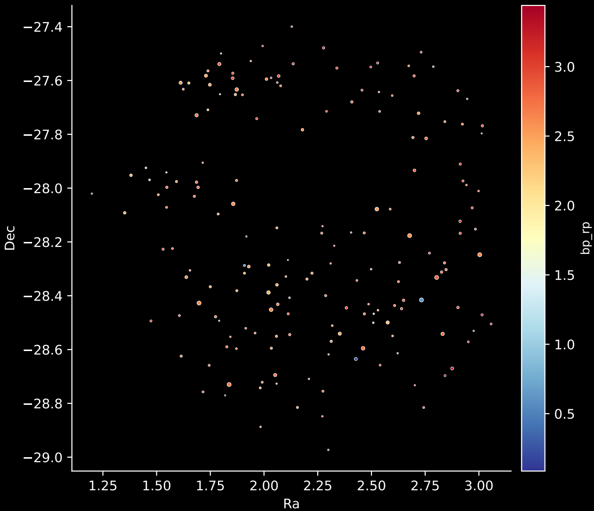
APOGEE DR17 Field: [359+04-O] Stars: 176
