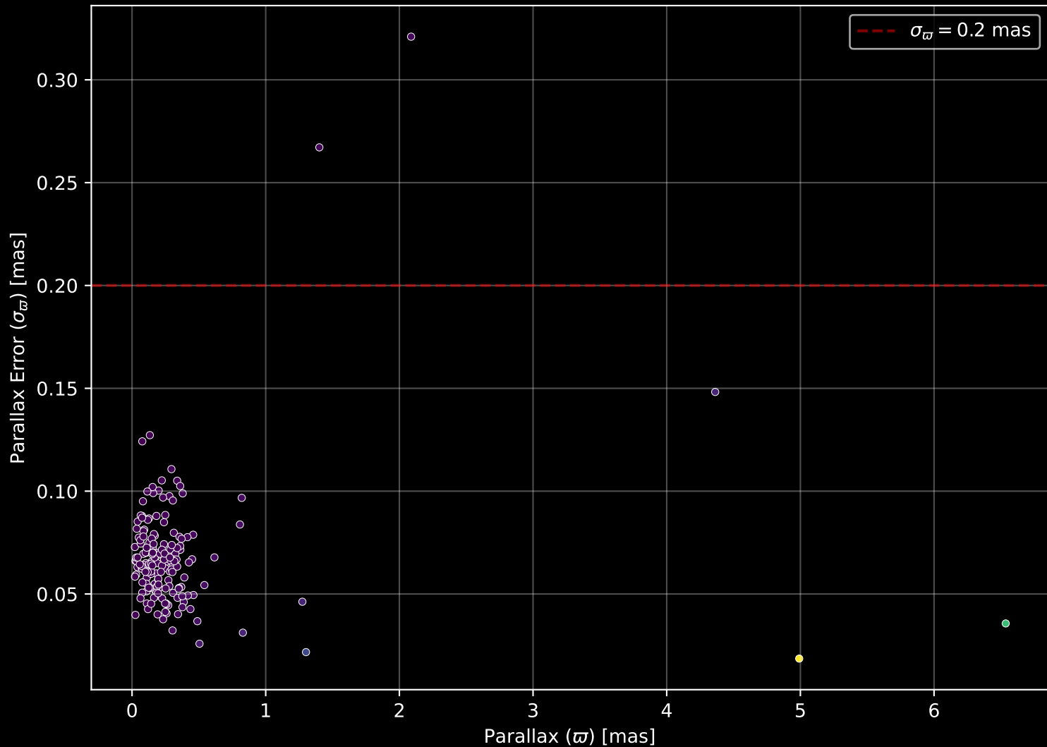
APOGEE DR17 Field: [359+04-O] Parallax Quality (n= 176)
